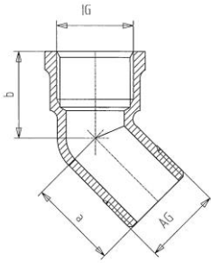
45° elbow, female/male
